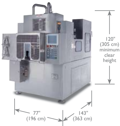
Model 624 dimensions
